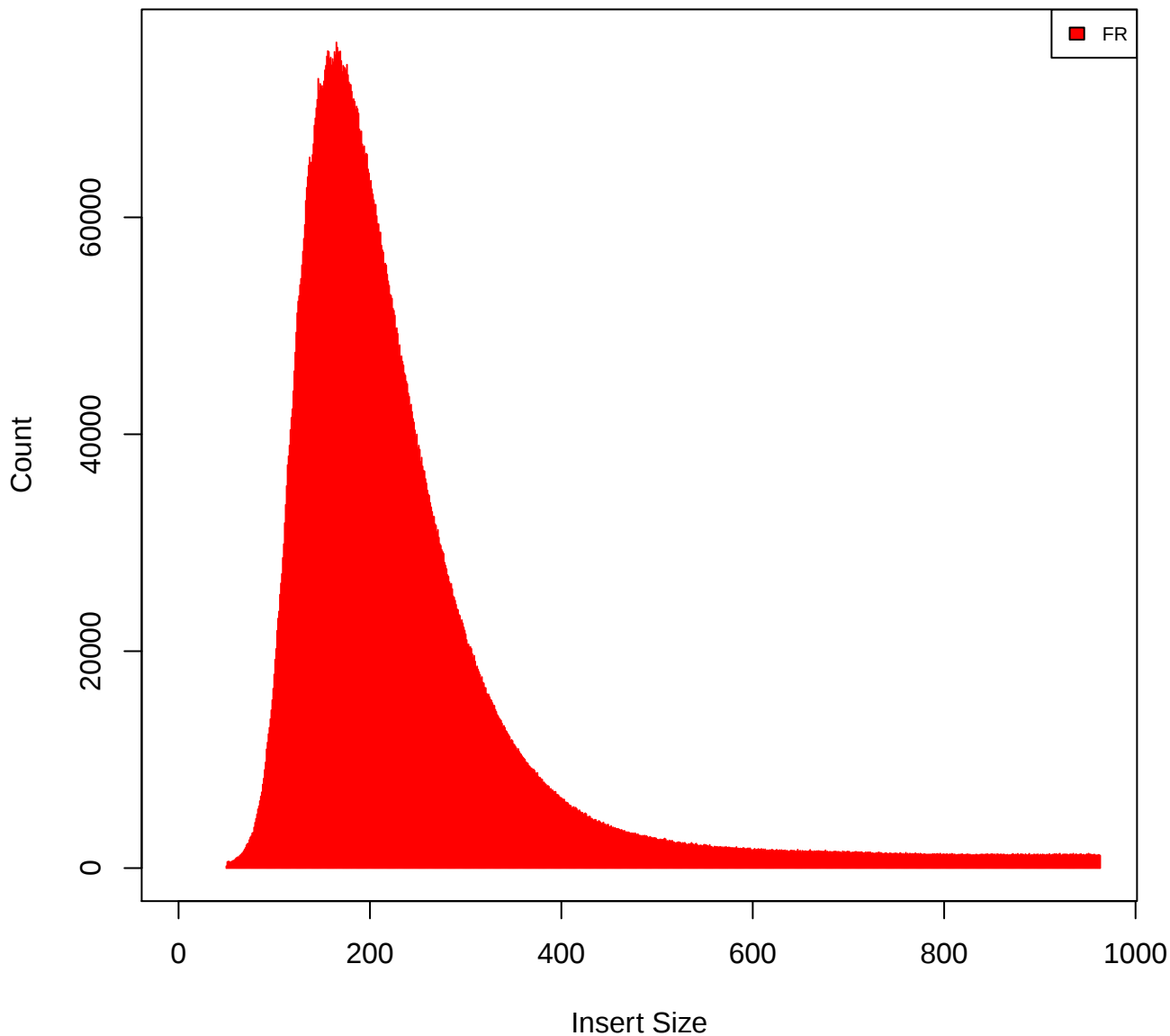
Insert Size Histogram for All_Reads in file G123_M8_primary_unique.bam
