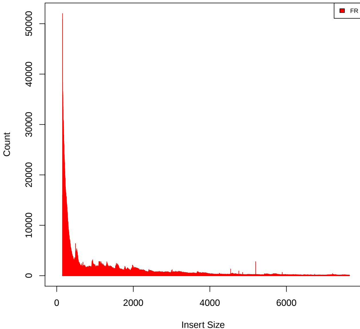
Insert Size Histogram for All_Reads in file G167_M1_primary_unique.bam
