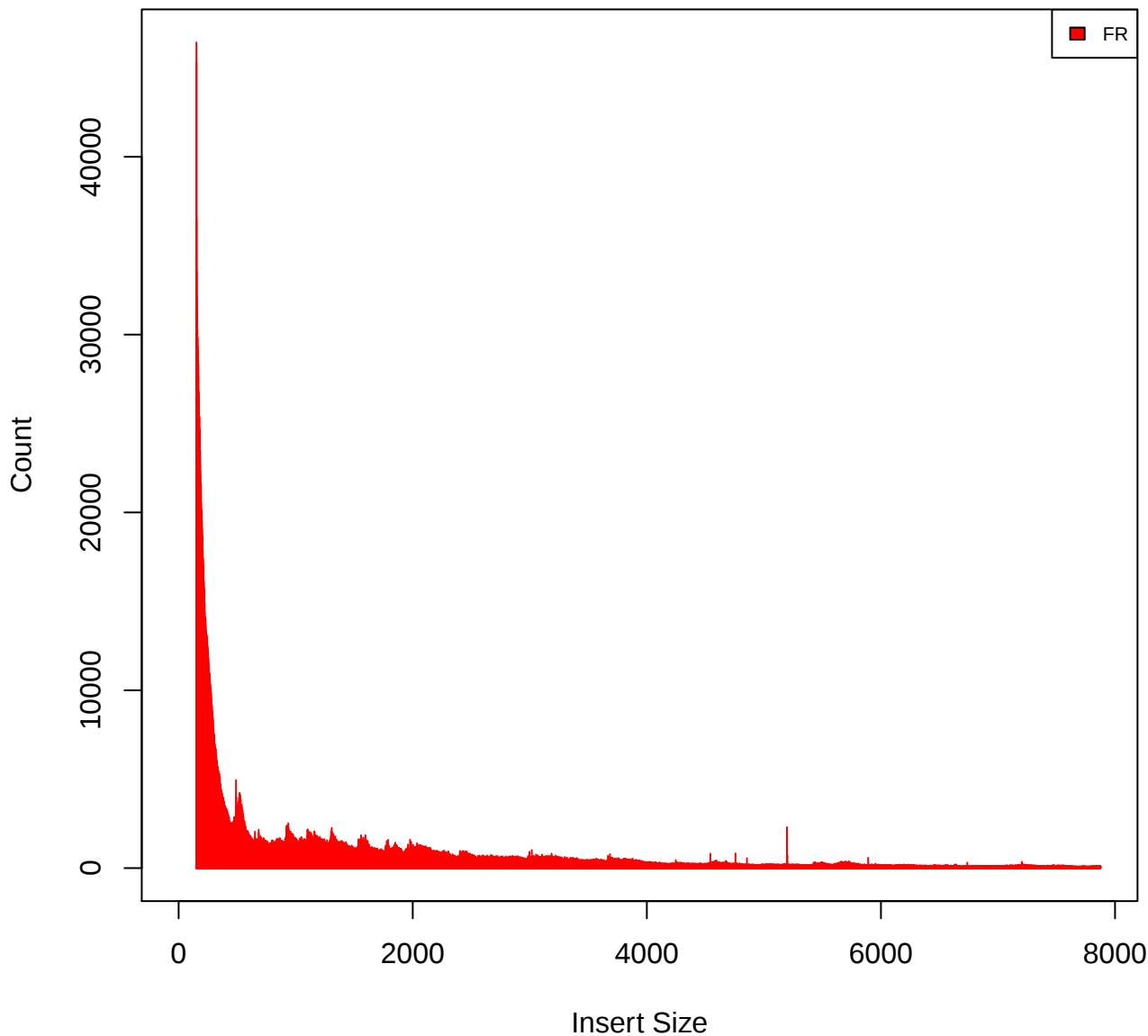
Insert Size Histogram for All_Reads in file G167_M2_primary_unique.bam
