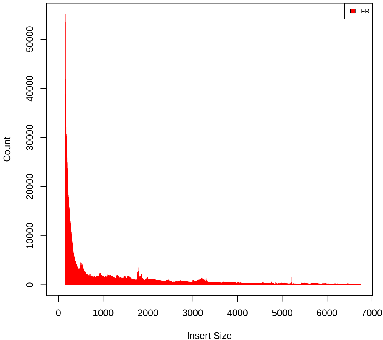
Insert Size Histogram for All_Reads in file G167_M7_primary_unique.bam
