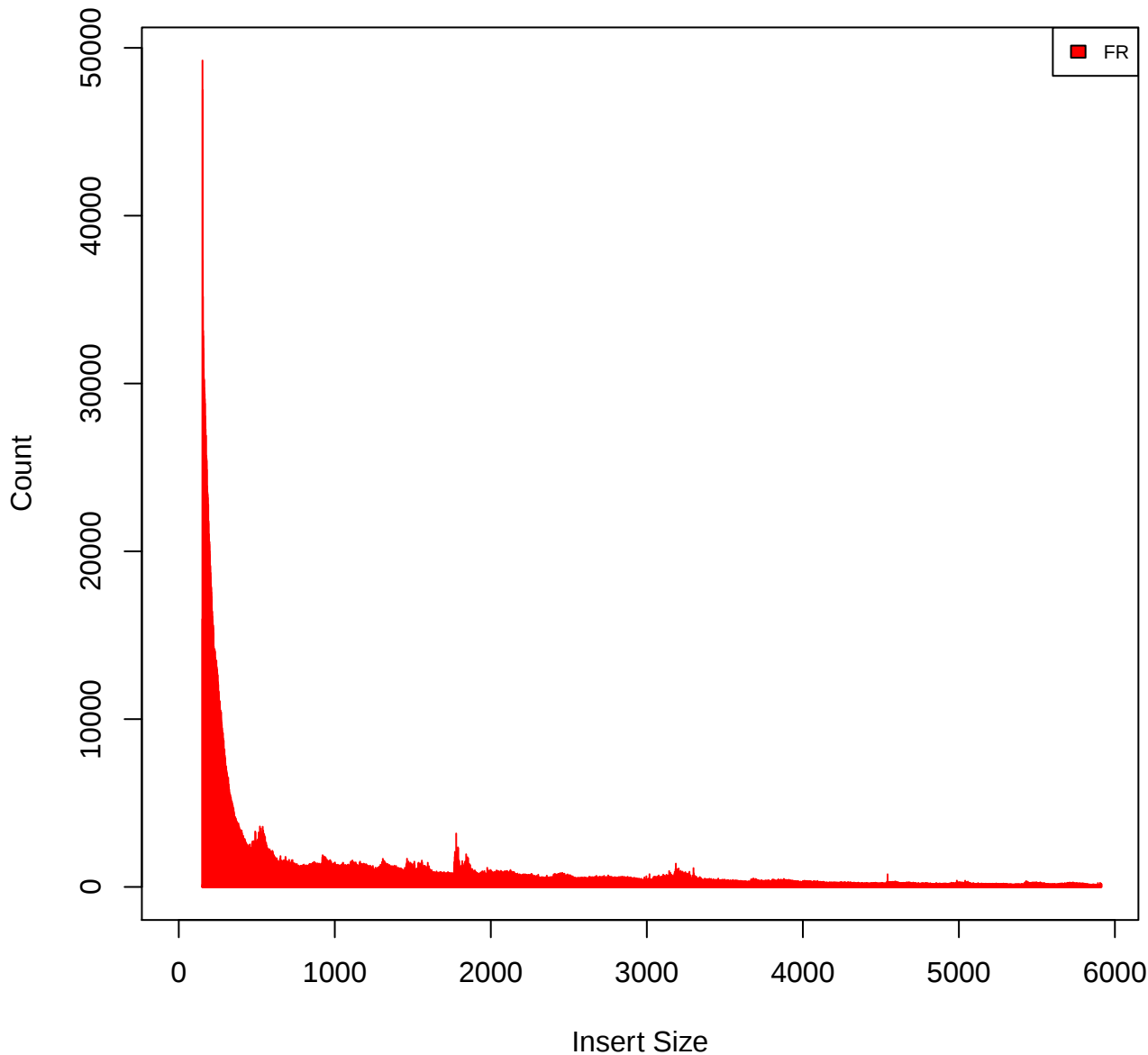
Insert Size Histogram for All_Reads in file G167_M10_primary_unique.bam
