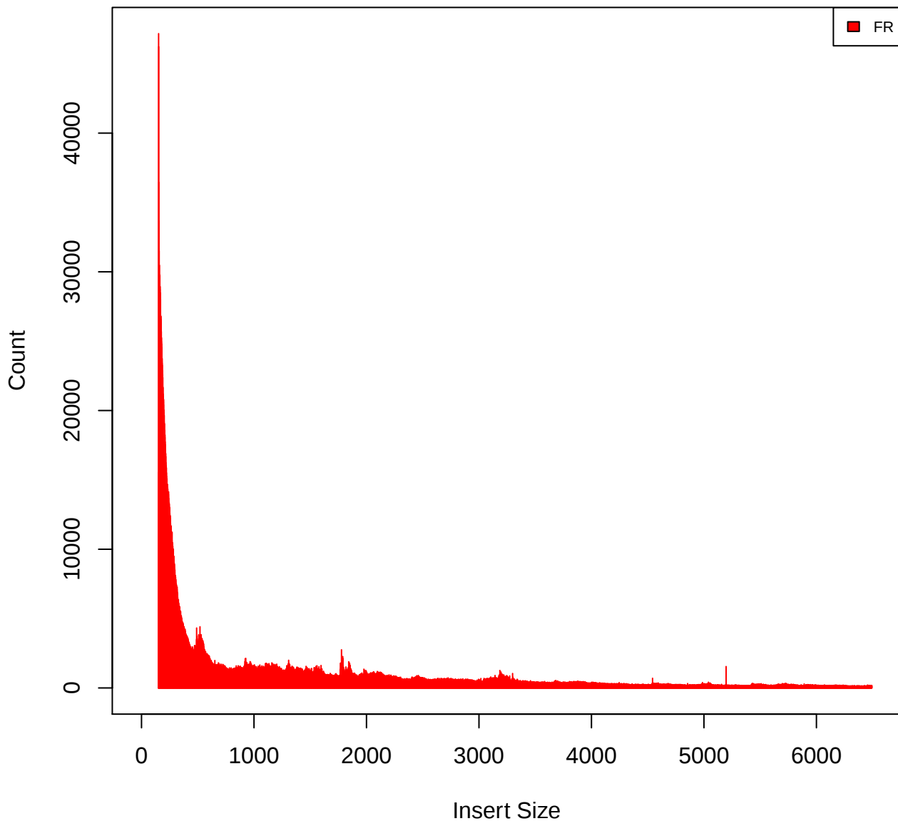
Insert Size Histogram for All_Reads in file G167_M8_primary_unique.bam
