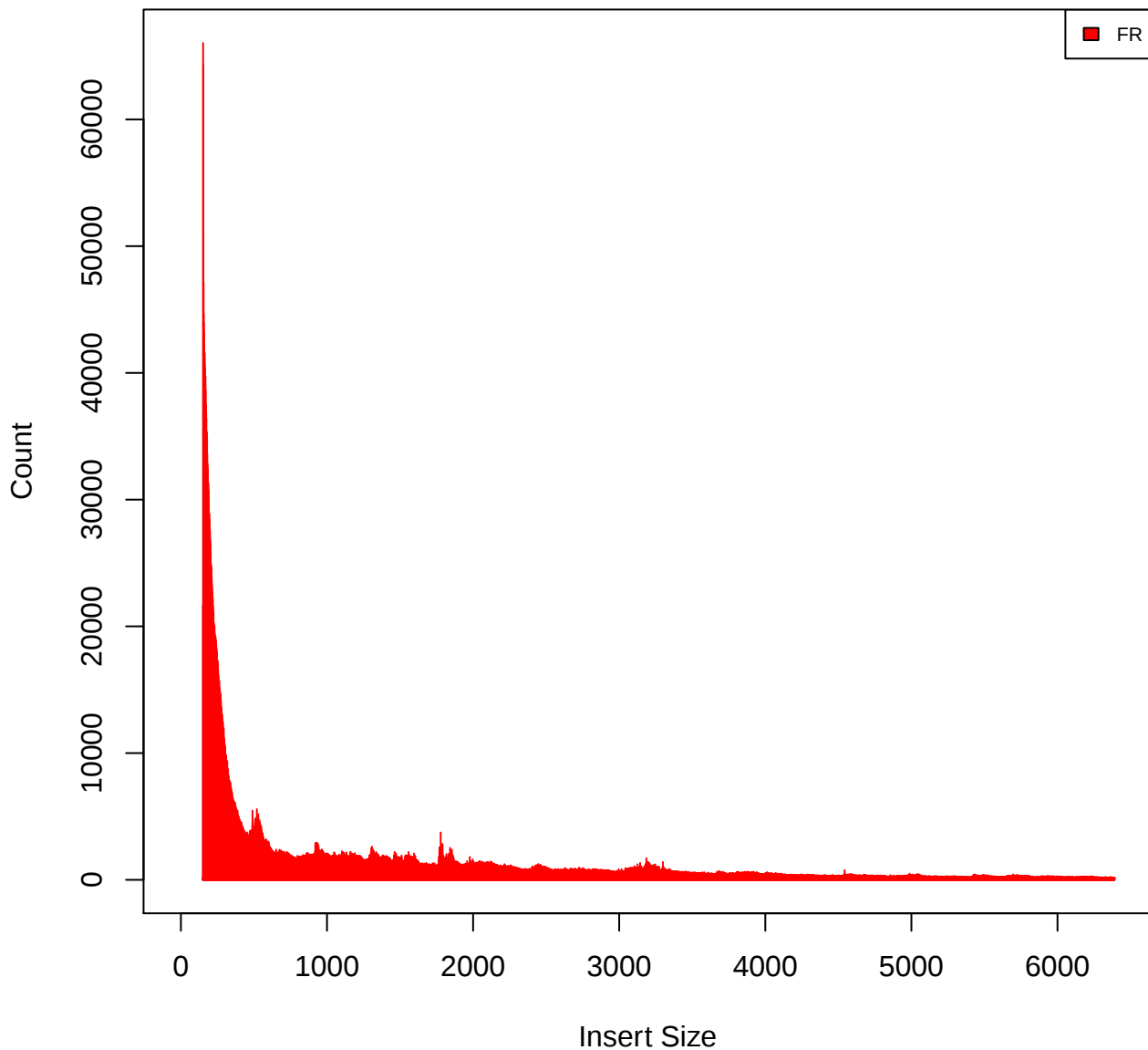
Insert Size Histogram for All_Reads in file G167_M12_primary_unique.bam
