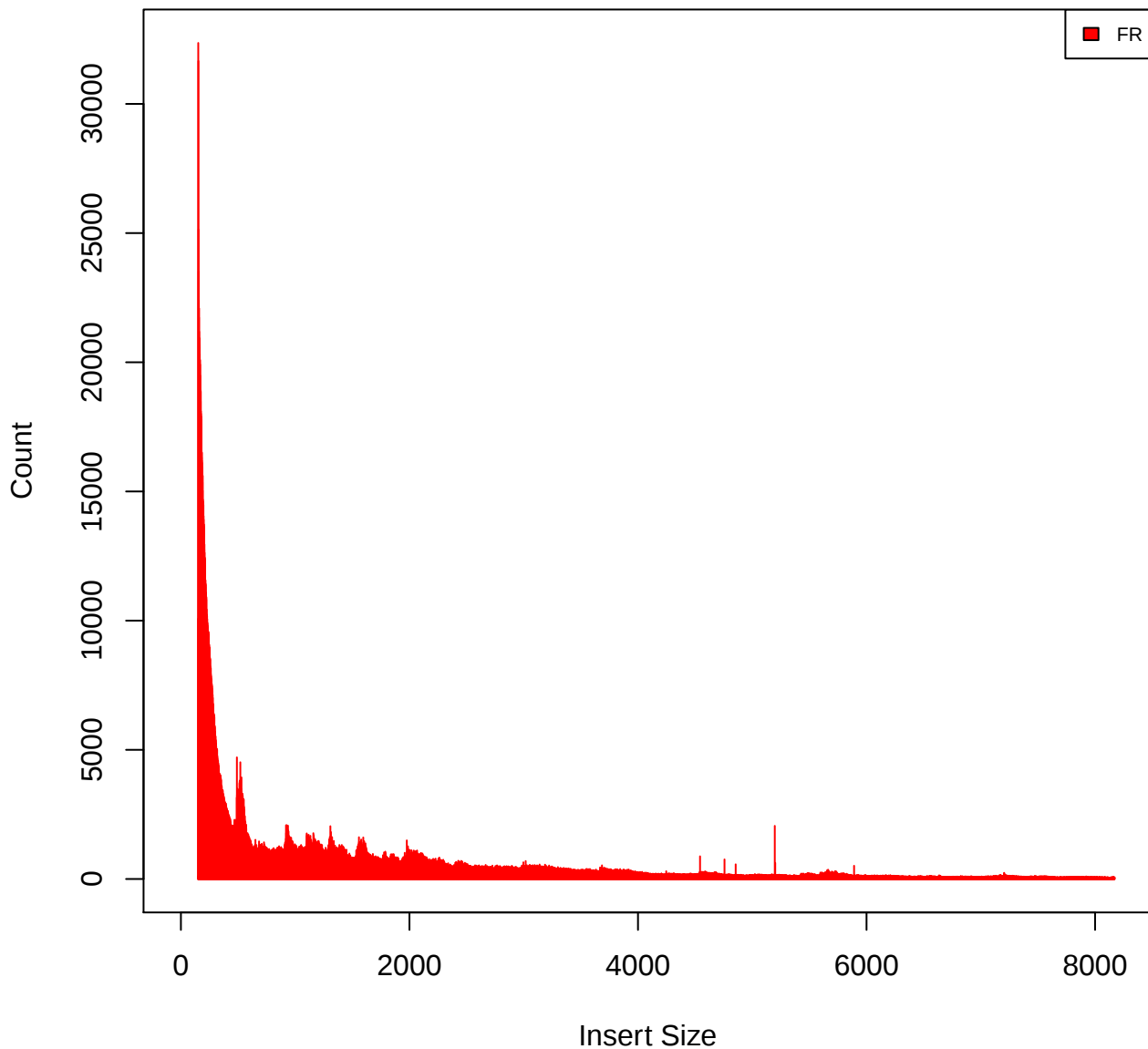
Insert Size Histogram for All_Reads in file G167_M3_primary_unique.bam
