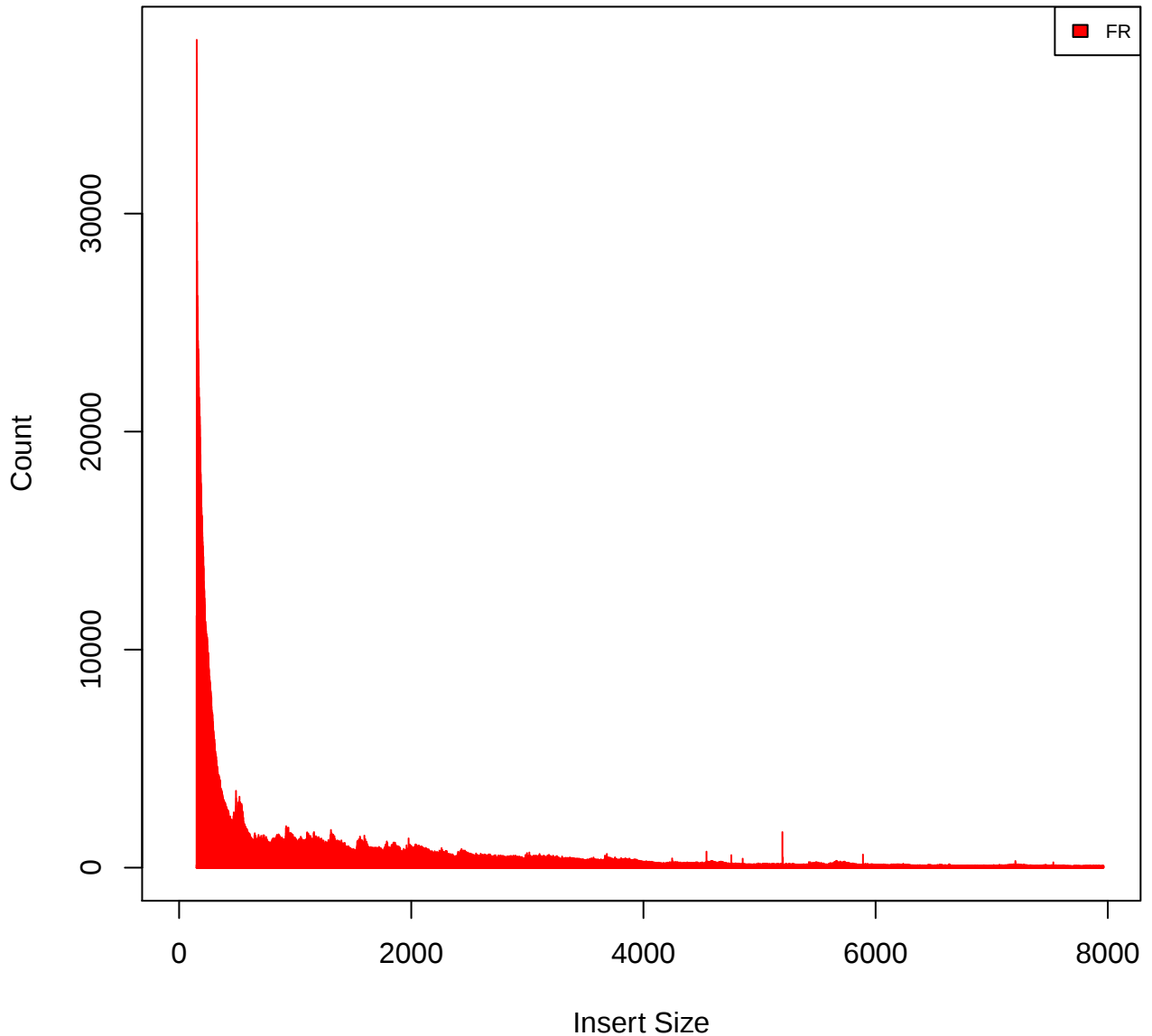
Insert Size Histogram for All_Reads in file G167_M6_primary_unique.bam
