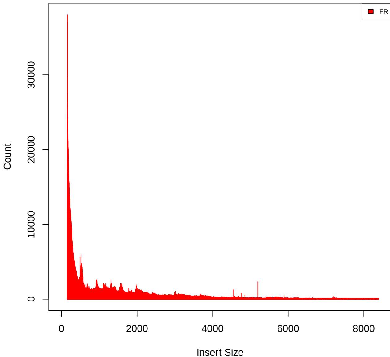
Insert Size Histogram for All_Reads in file G167_M5_primary_unique.bam
