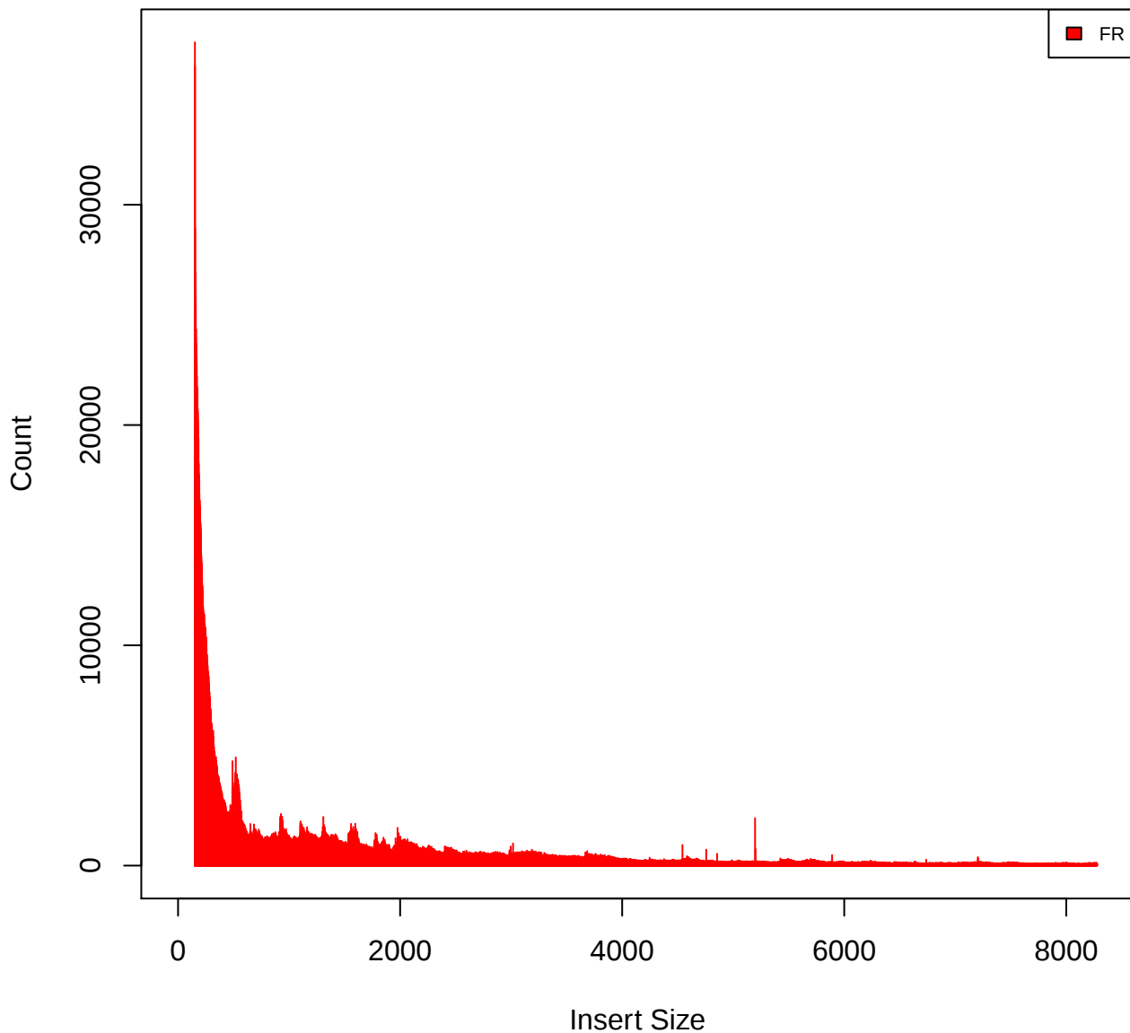
Insert Size Histogram for All_Reads in file G167_M4_primary_unique.bam
